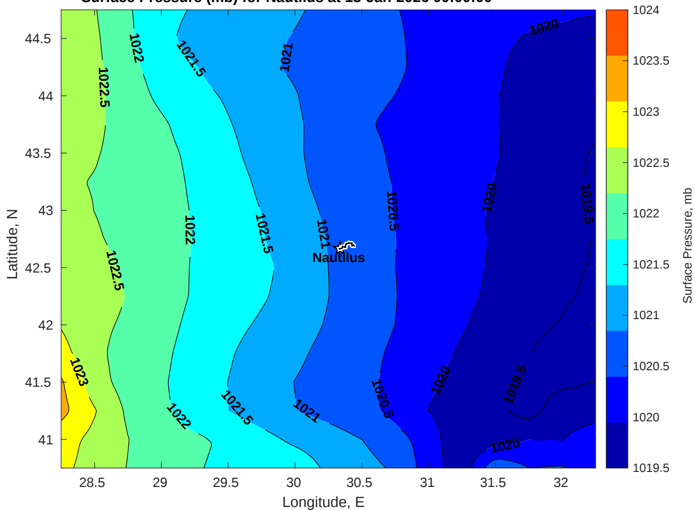
Surface Pressure (mb) for Nautilus at 13-Jan-2026 00:00:00
