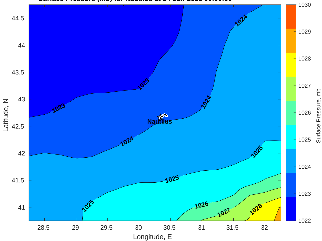
Surface Pressure (mb) for Nautilus at 14-Jan-2026 00:00:00
