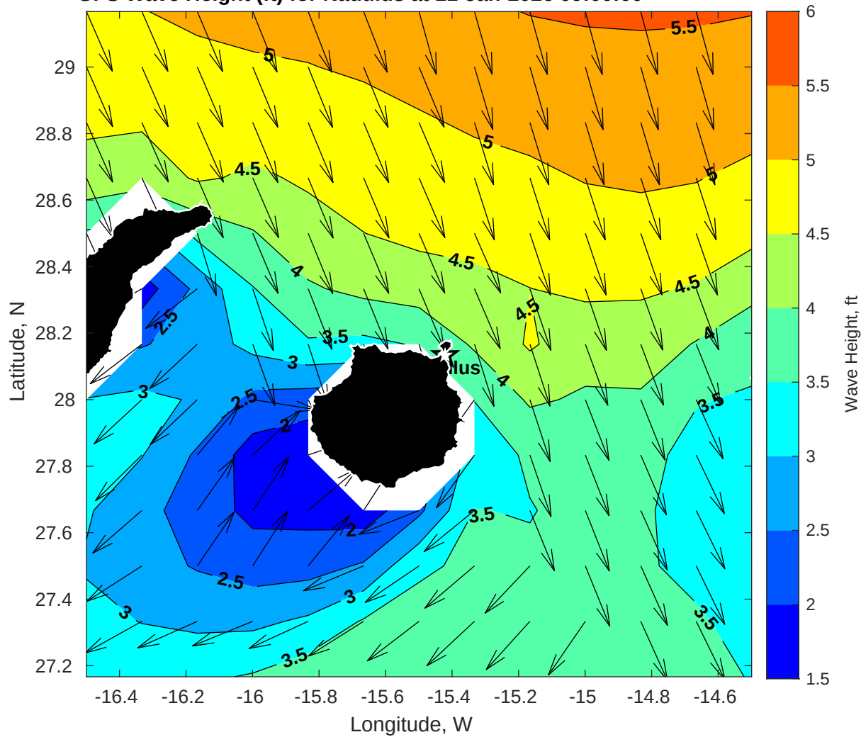
GFS Wave Height (ft) for Nautilus at 11-Jan-2026 09:00:00
