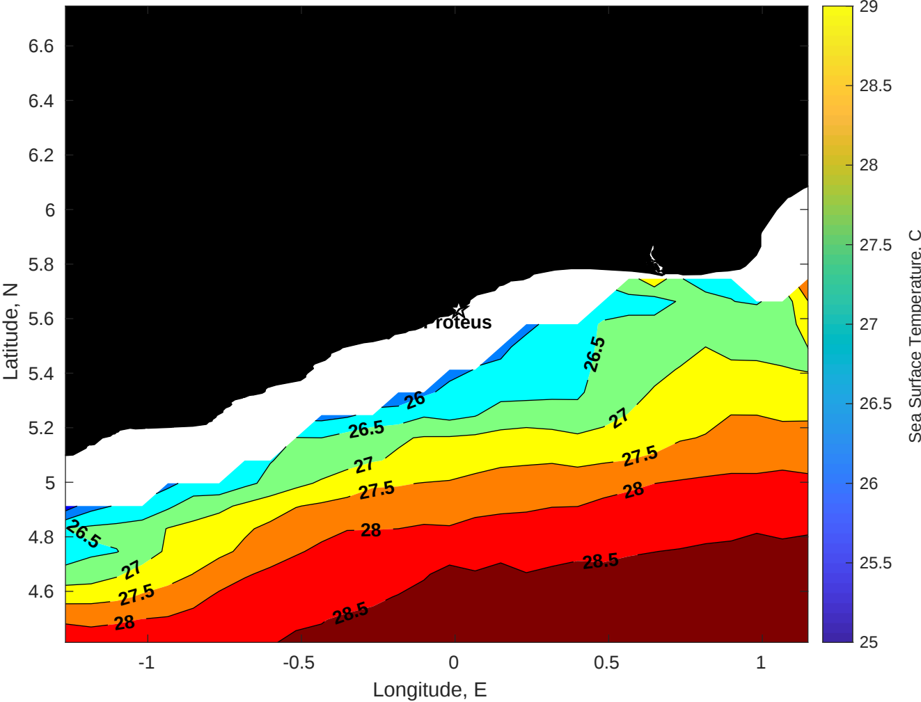
SST for Proteus at 11-Jan-2026 00:00:00
