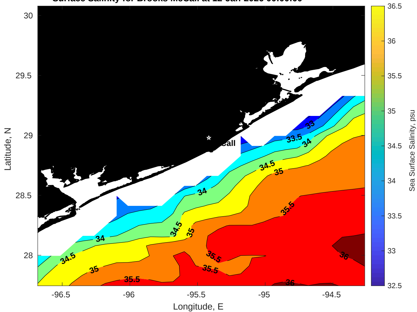
Surface Salinity for Brooks McCall at 12-Jan-2026 00:00:00
