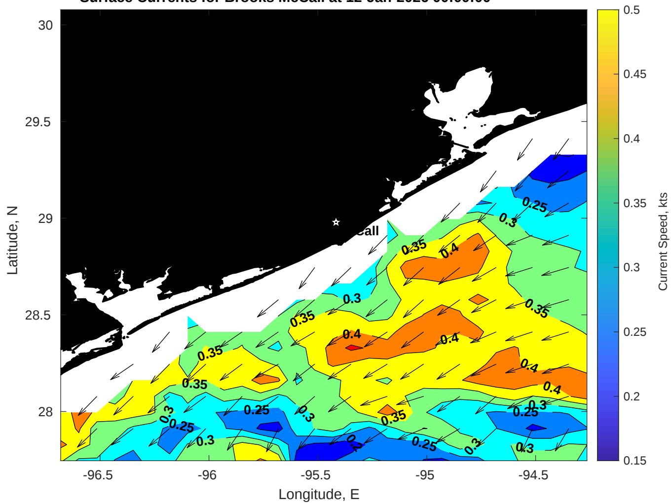
Surface Currents for Brooks McCall at 12-Jan-2026 00:00:00
