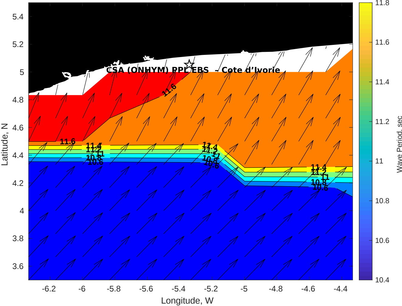
GFS Wave Period (sec) for CSA (ONHYM) PPL EBS - Cote d'Ivoire at 13-Jan-2026 09:00:00
