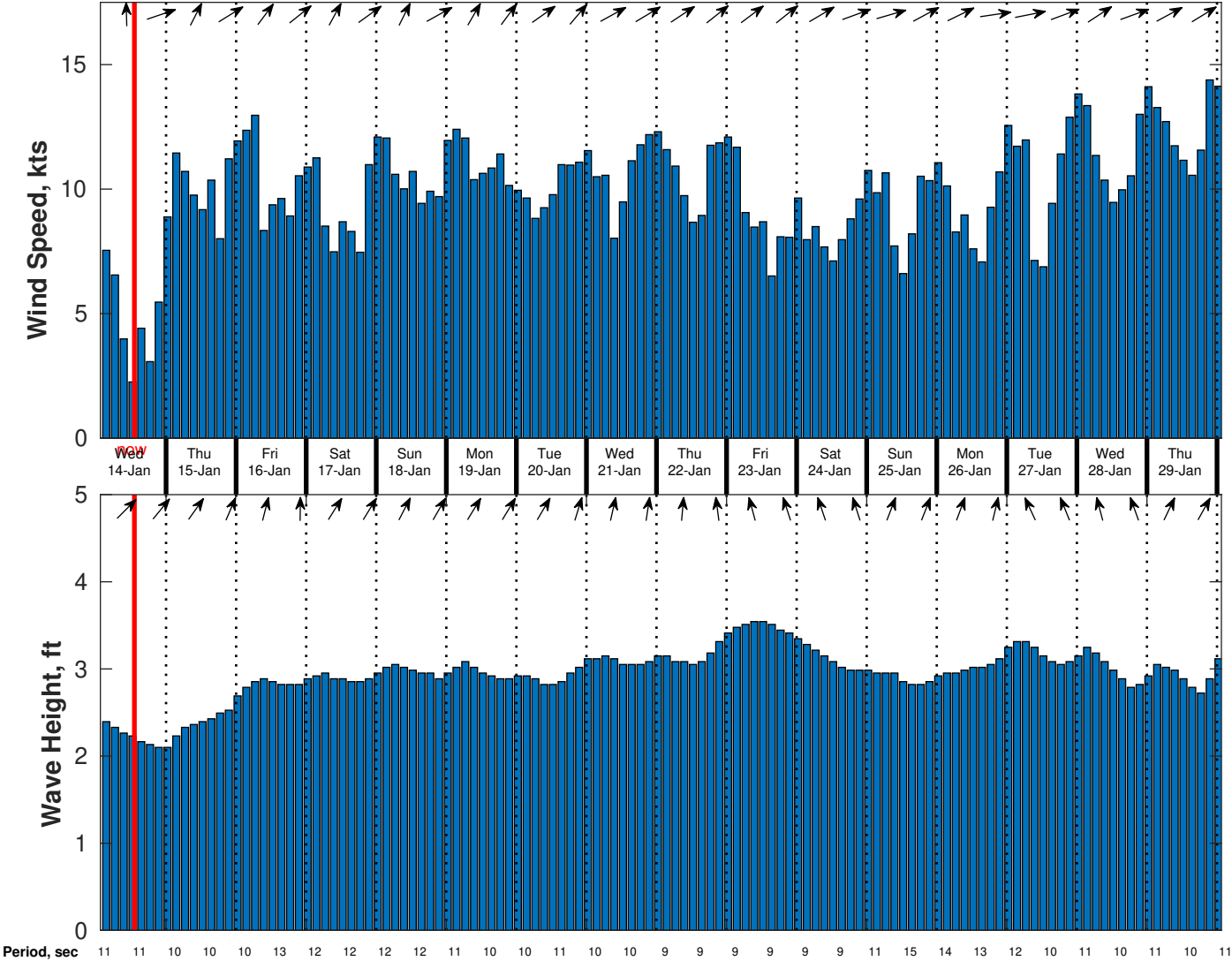
Wind & Wave Forecast for CSA (ONHYM) PPL EBS - Ghana from 13-Jan-2026 02:00:00 to 29-Jan-2026 02:00:00
