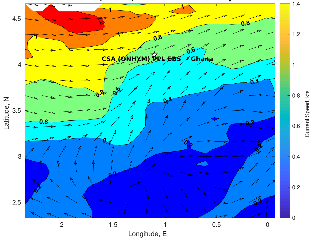
Surface Currents for CSA (ONHYM) PPL EBS - Ghana at 12-Jan-2026 00:00:00
