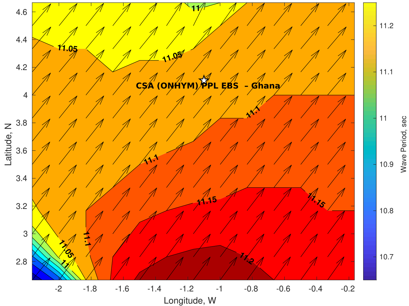
GFS Wave Period (sec) for CSA (ONHYM) PPL EBS - Ghana at 13-Jan-2026 09:00:00
