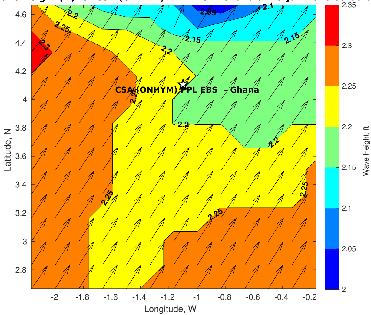
GFS Wave Height (ft) for CSA (ONHYM) PPL EBS - Ghana at 13-Jan-2026 09:00:00
