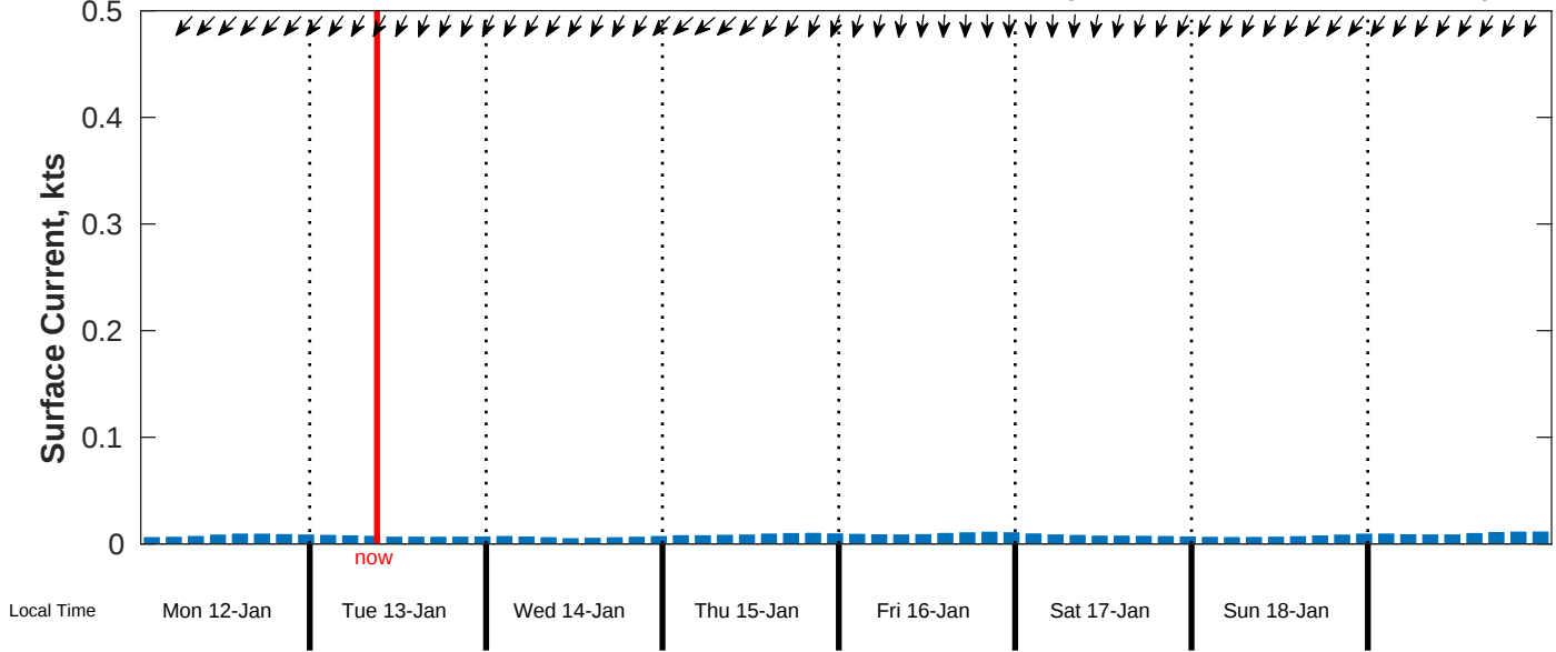
Surface Current Forecast for CSA (ONHYM) PPL EBS - Ghana from 12-Jan-2026 00:00:00 to 20-Jan-2026 00:00:00
