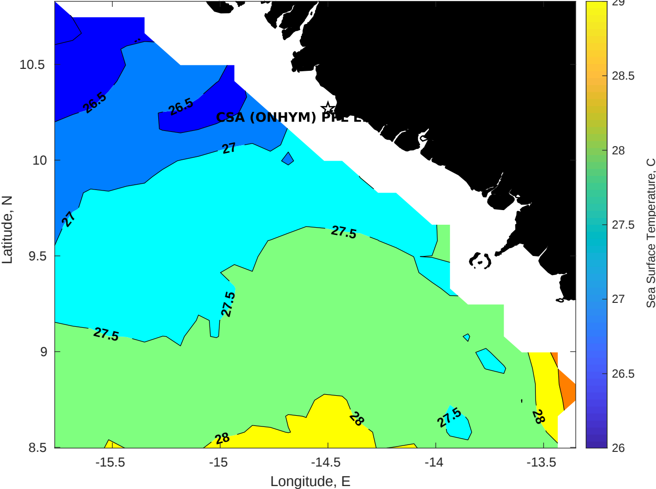
SST for CSA (ONHYM) PPL EBS - Guinea at 12-Jan-2026 00:00:00
