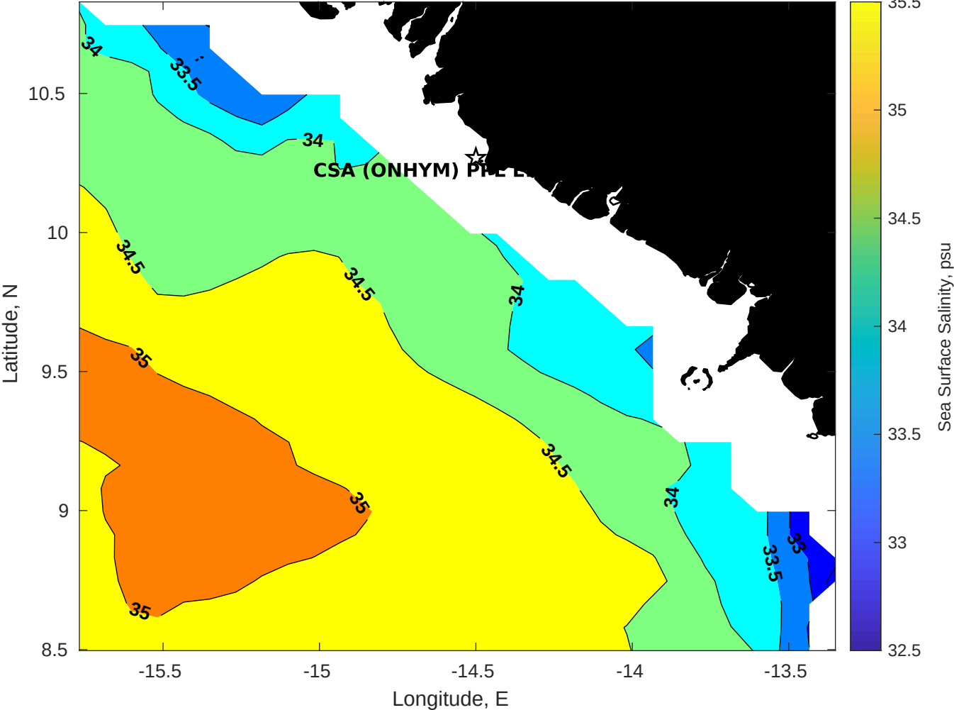
Surface Salinity for CSA (ONHYM) PPL EBS - Guinea at 12-Jan-2026 00:00:00
