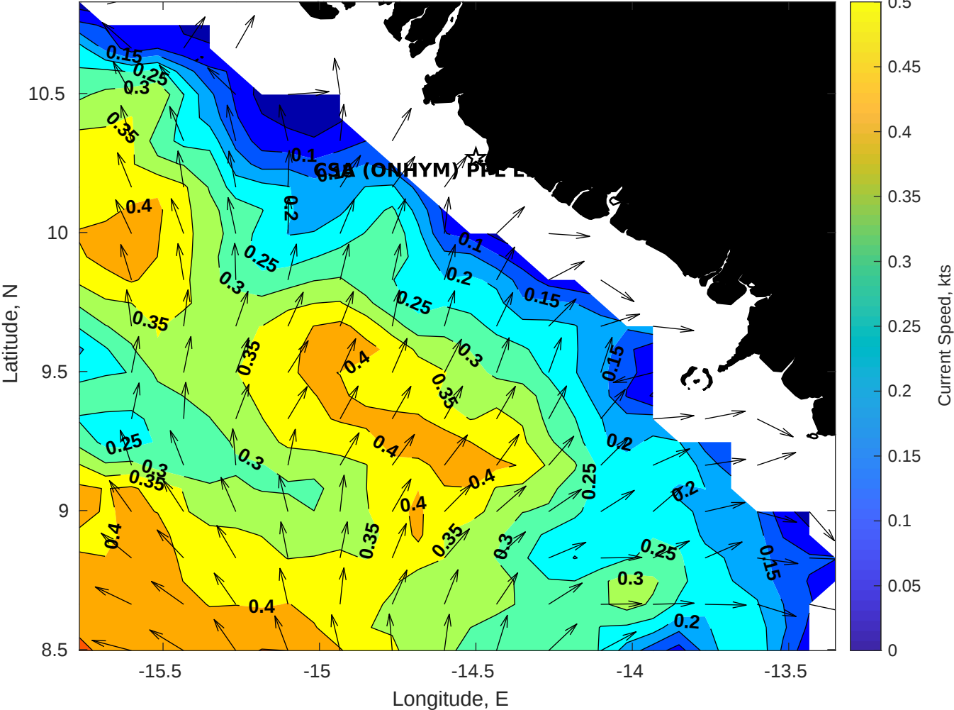
Surface Currents for CSA (ONHYM) PPL EBS - Guinea at 12-Jan-2026 00:00:00
