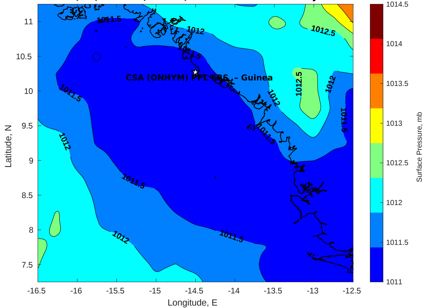
Surface Pressure (mb) for CSA (ONHYM) PPL EBS - Guinea at 13-Jan-2026 00:00:00
