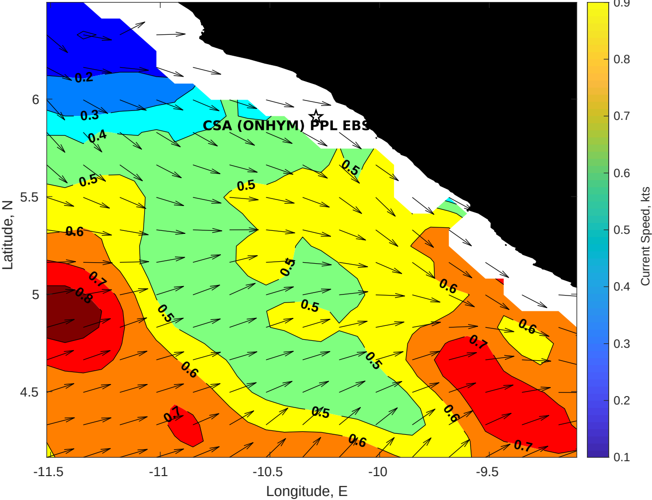
Surface Currents for CSA (ONHYM) PPL EBS - Liberia at 12-Jan-2026 00:00:00
