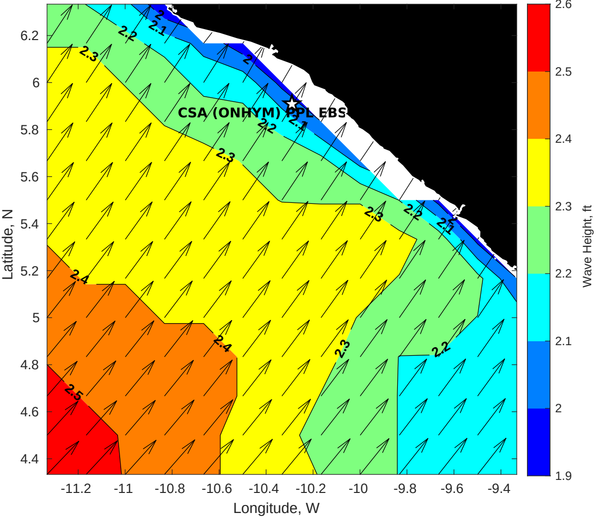
GFS Wave Height (ft) for CSA (ONHYM) PPL EBS - Liberia at 13-Jan-2026 09:00:00
