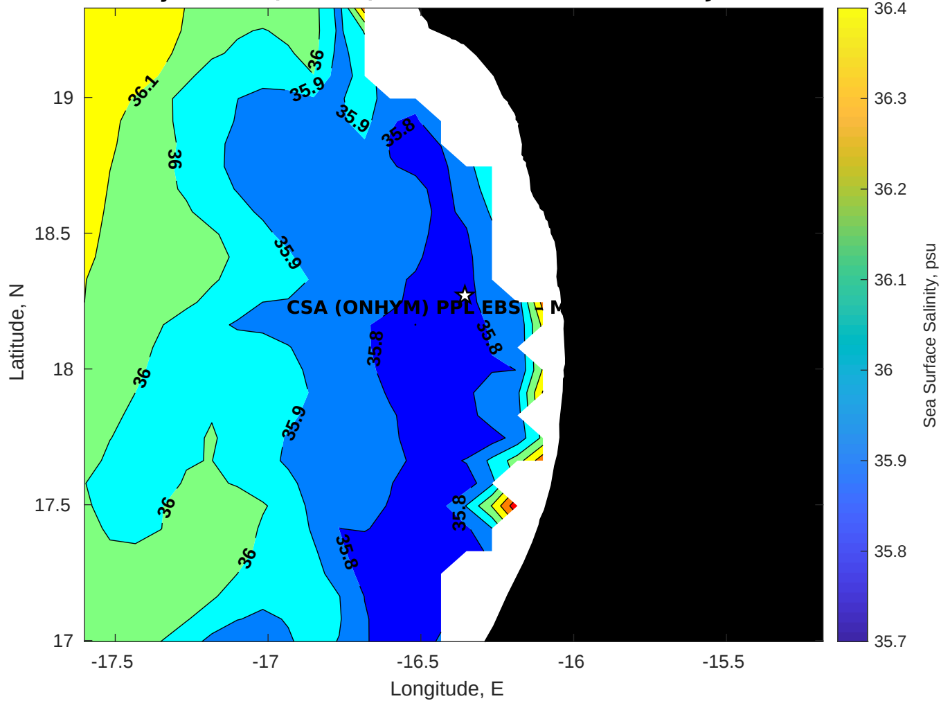
Surface Salinity for CSA (ONHYM) PPL EBS - Mauritania at 12-Jan-2026 00:00:00
