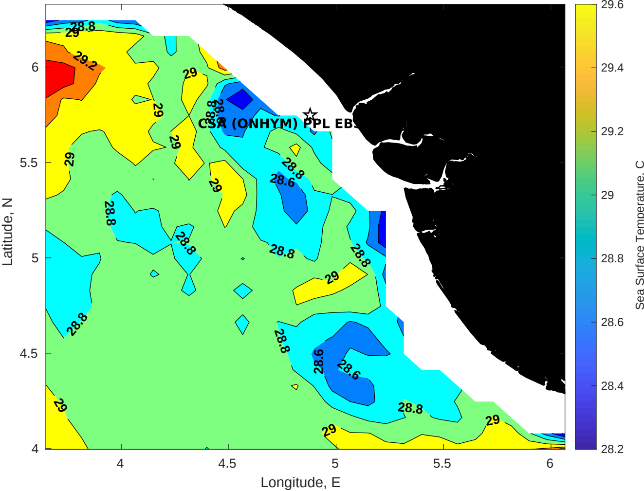
SST for CSA (ONHYM) PPL EBS - Nigeria at 12-Jan-2026 00:00:00
