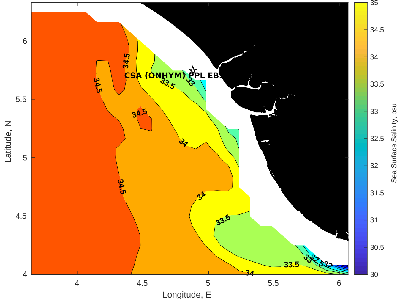
Surface Salinity for CSA (ONHYM) PPL EBS - Nigeria at 12-Jan-2026 00:00:00
