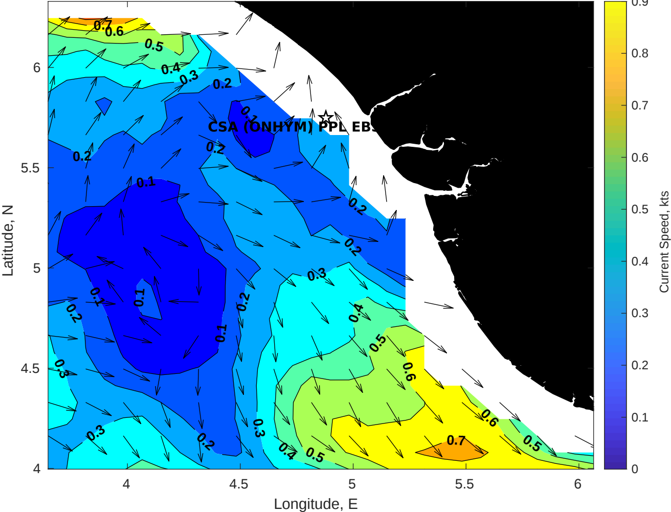
Surface Currents for CSA (ONHYM) PPL EBS - Nigeria at 12-Jan-2026 00:00:00
