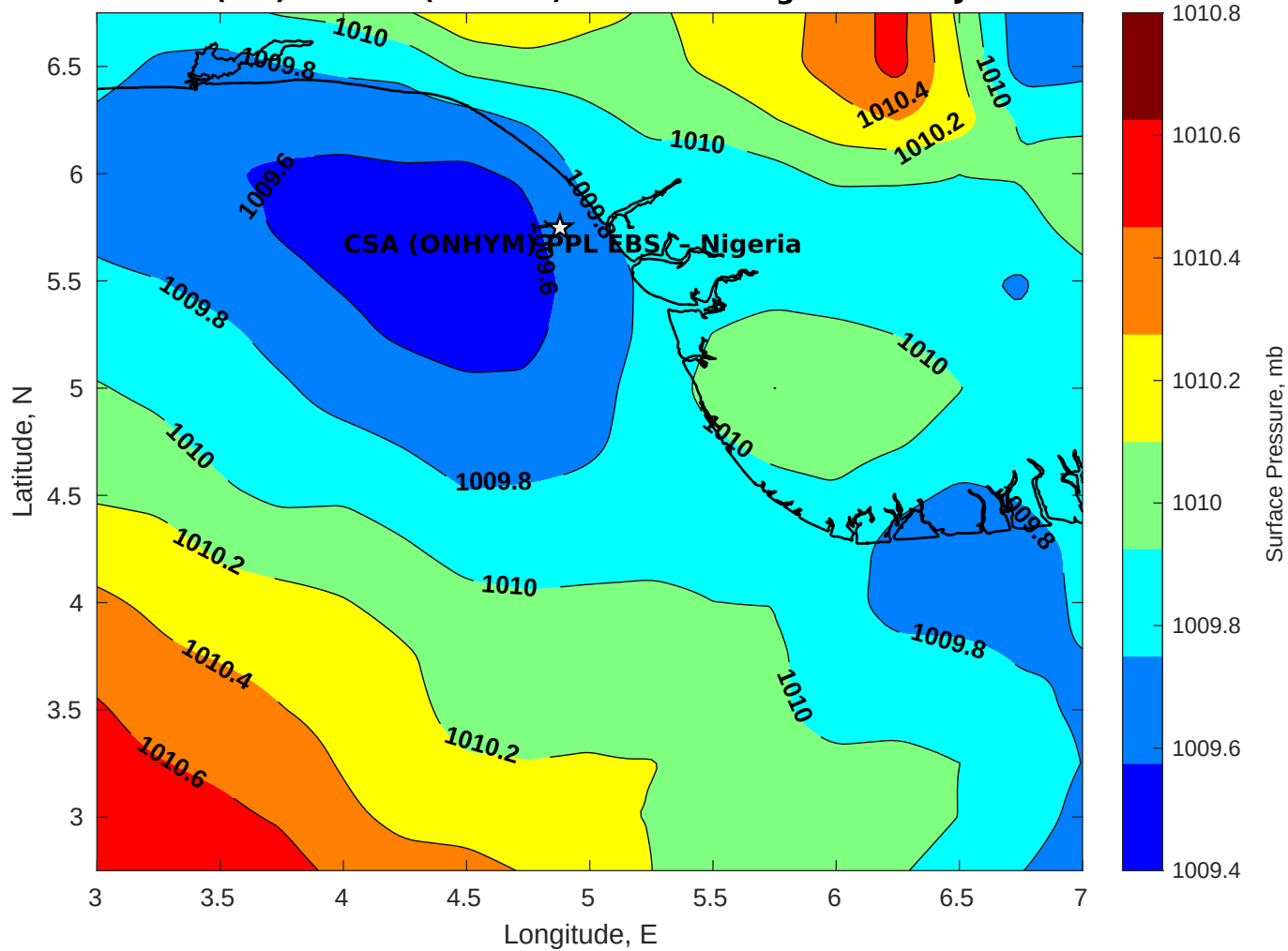
Surface Pressure (mb) for CSA (ONHYM) PPL EBS - Nigeria at 13-Jan-2026 00:00:00
