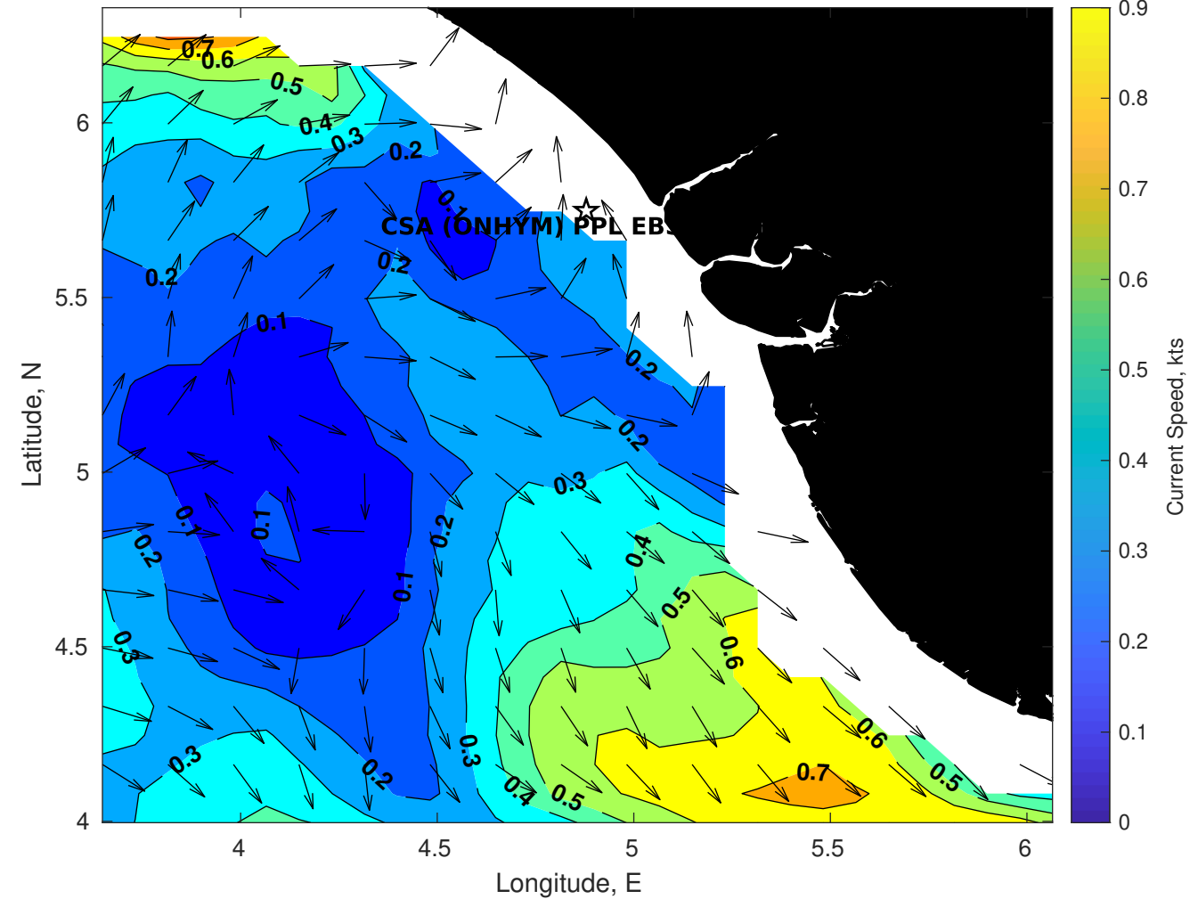
Surface Currents for CSA (ONHYM) PPL EBS - Nigeria at 12-Jan-2026 00:00:00
