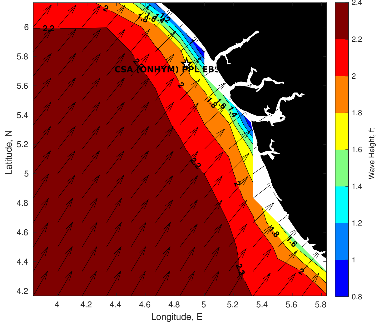
GFS Wave Height (ft) for CSA (ONHYM) PPL EBS - Nigeria at 13-Jan-2026 09:00:00
