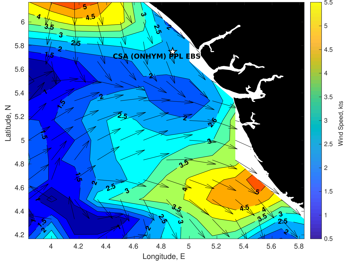
GFS Winds (kts) for CSA (ONHYM) PPL EBS - Nigeria at 13-Jan-2026 09:00:00
