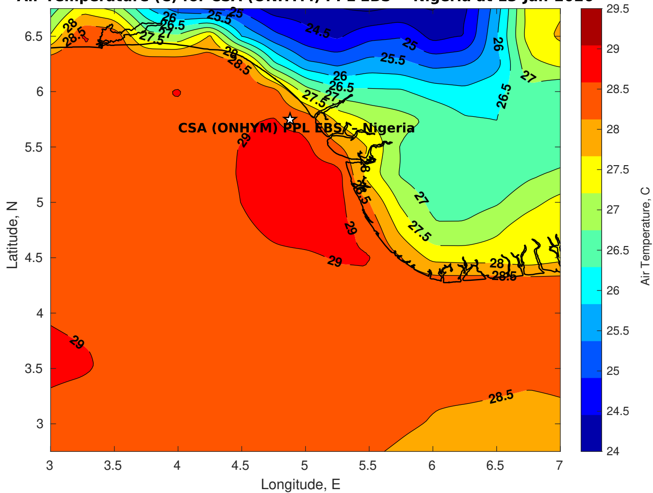
Air Temperature (C) for CSA (ONHYM) PPL EBS - Nigeria at 13-Jan-2026
