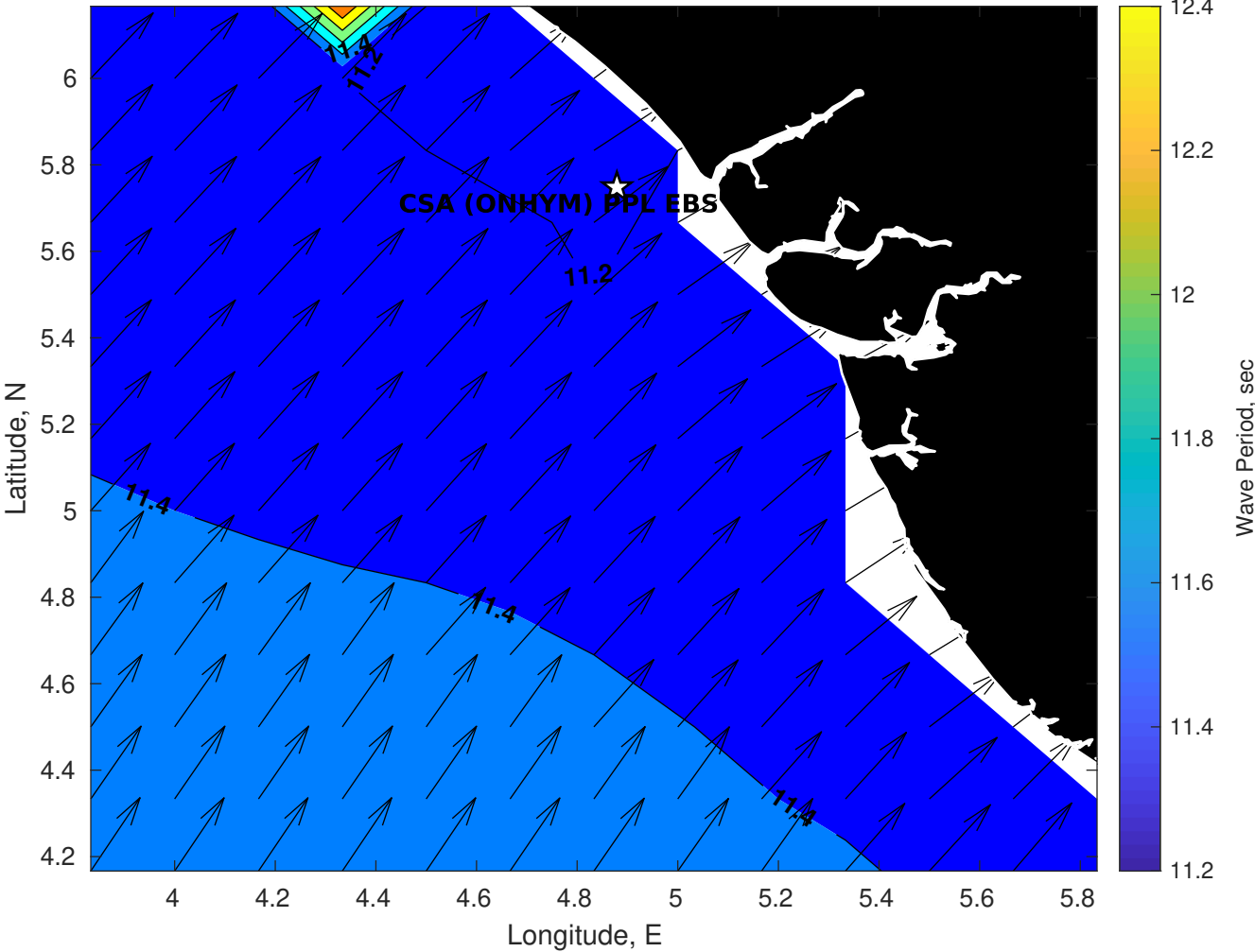
GFS Wave Period (sec) for CSA (ONHYM) PPL EBS - Nigeria at 13-Jan-2026 09:00:00
