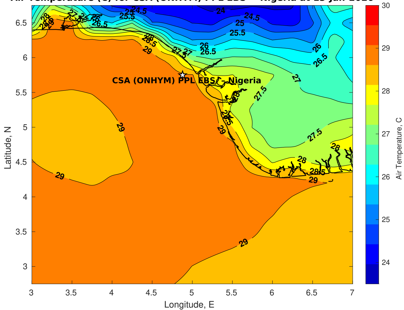
Air Temperature (C) for CSA (ONHYM) PPL EBS - Nigeria at 13-Jan-2026
