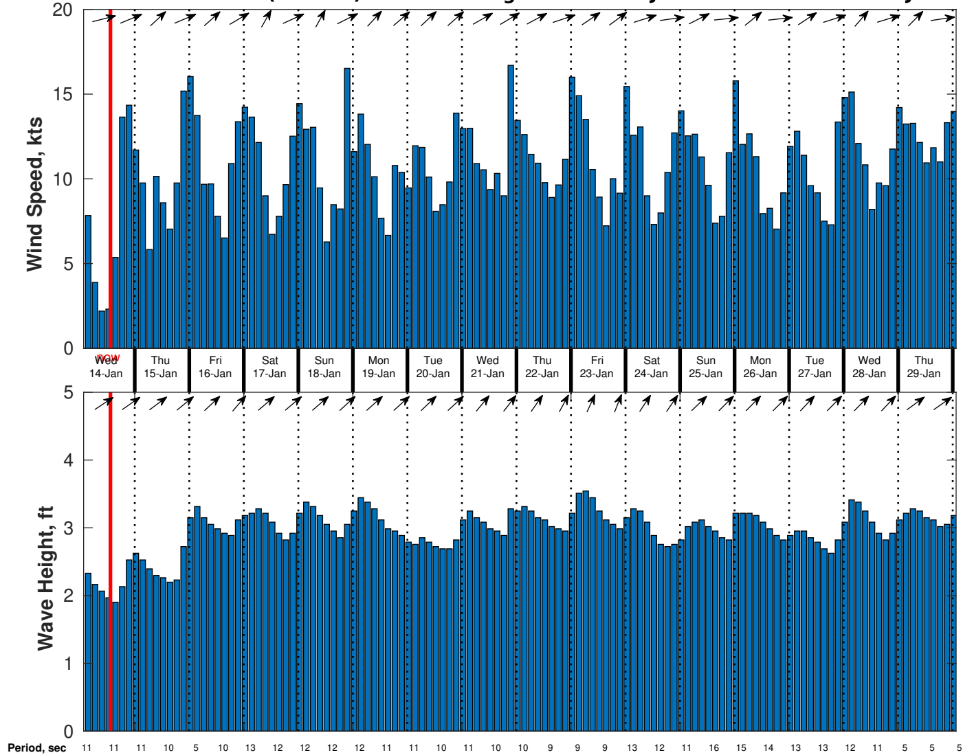
Wind & Wave Forecast for CSA (ONHYM) PPL EBS - Nigeria from 13-Jan-2026 02:00:00 to 29-Jan-2026 02:00:00
