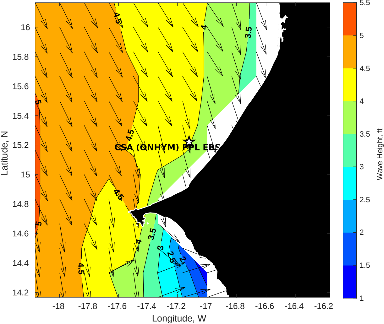
GFS Wave Height (ft) for CSA (ONHYM) PPL EBS - Senegal at 13-Jan-2026 09:00:00
