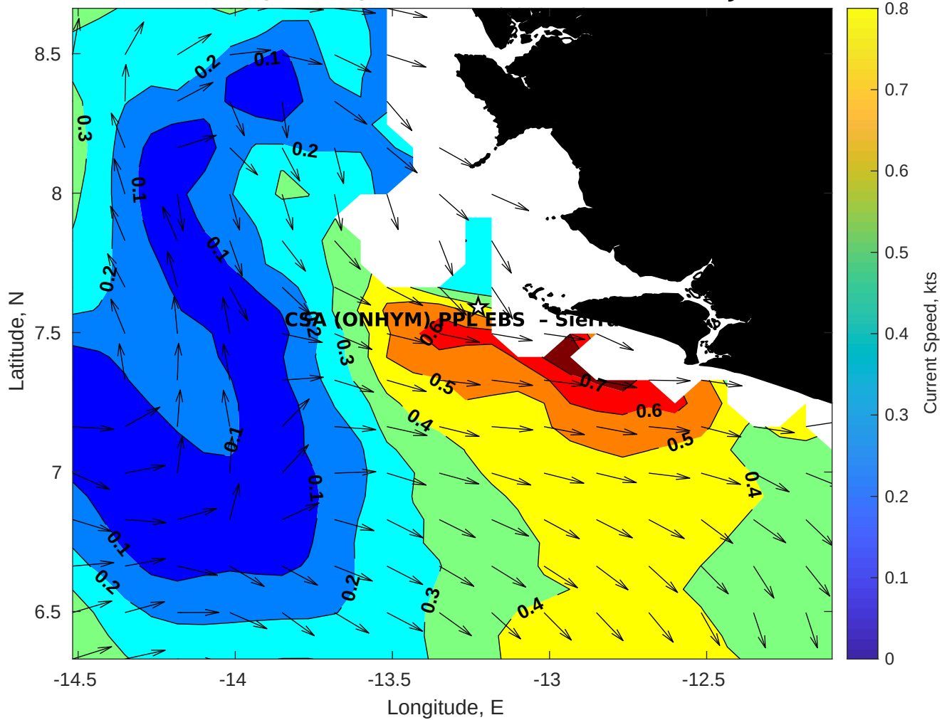
Surface Currents for CSA (ONHYM) PPL EBS - Sierra Leone at 12-Jan-2026 00:00:00
