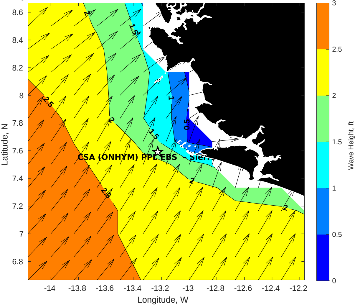
GFS Wave Height (ft) for CSA (ONHYM) PPL EBS - Sierra Leone at 13-Jan-2026 09:00:00
