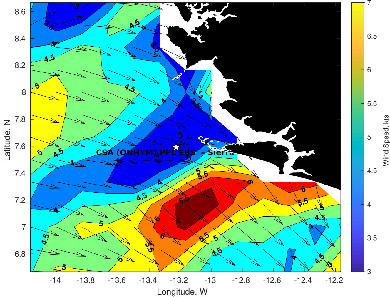
GFS Winds (kts) for CSA (ONHYM) PPL EBS - Sierra Leone at 13-Jan-2026 09:00:00
