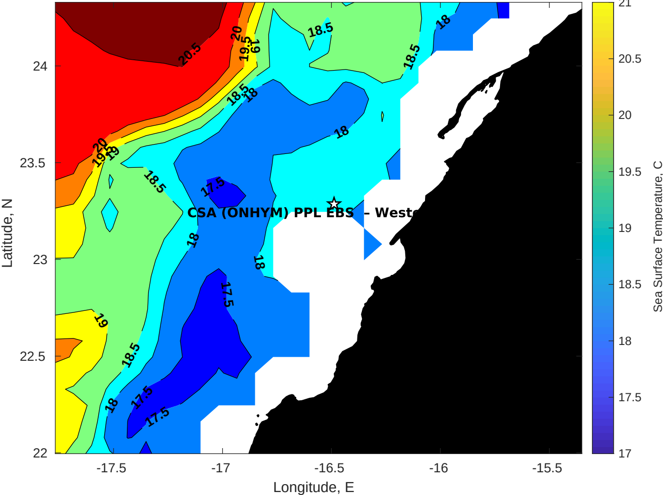
SST for CSA (ONHYM) PPL EBS - Western Sahara at 12-Jan-2026 00:00:00
