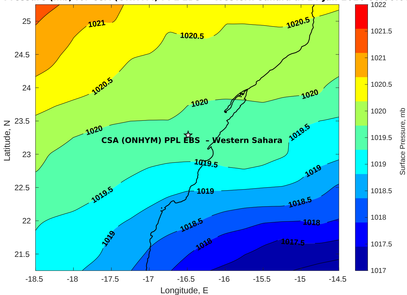
Surface Pressure (mb) for CSA (ONHYM) PPL EBS - Western Sahara at 14-Jan-2026 00:00:00
