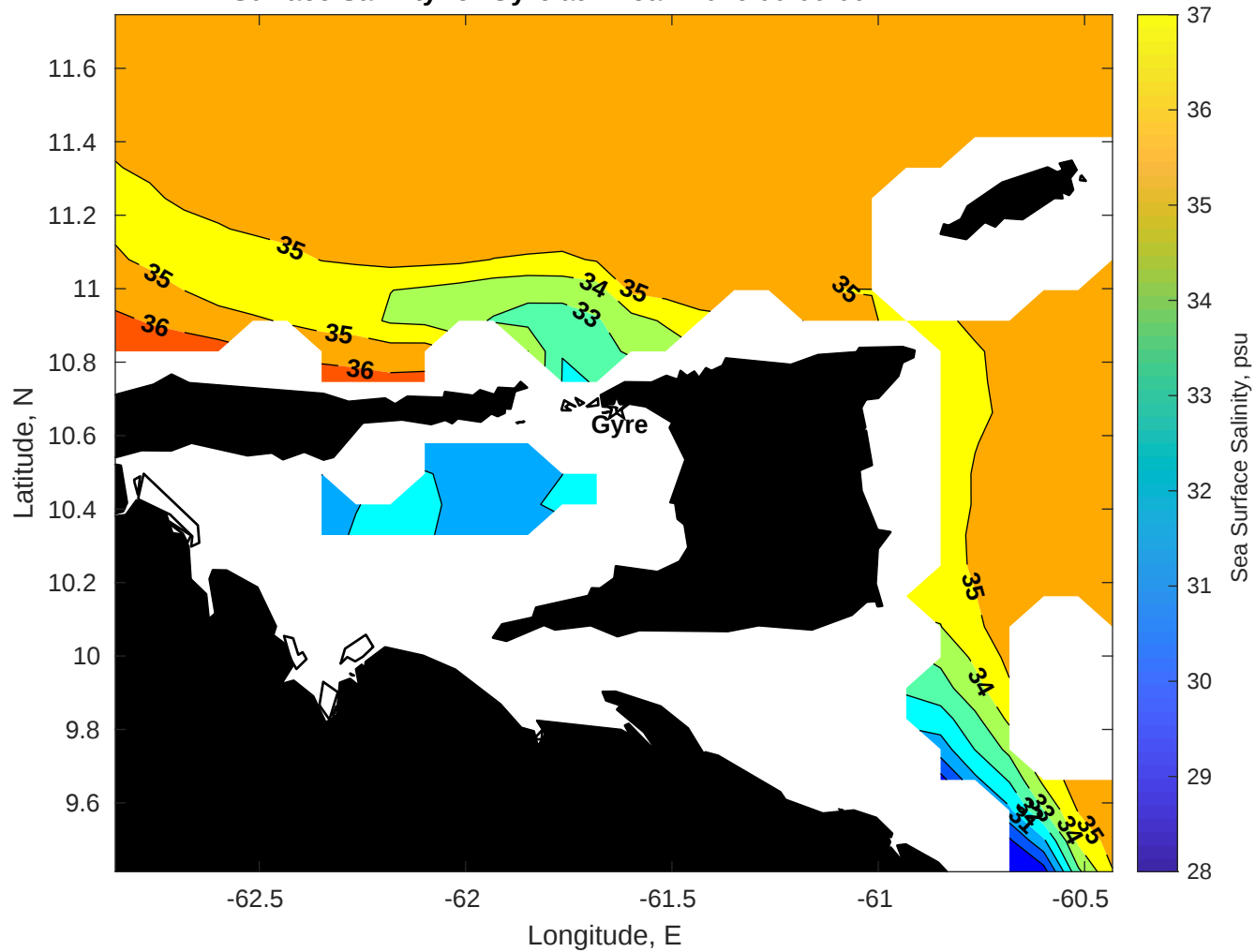
Surface Salinity for Gyre at 12-Jan-2026 00:00:00
