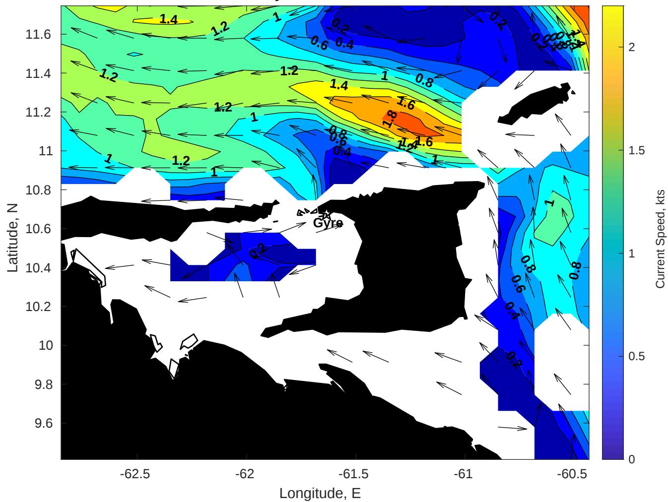
Surface Currents for Gyre at 12-Jan-2026 00:00:00
