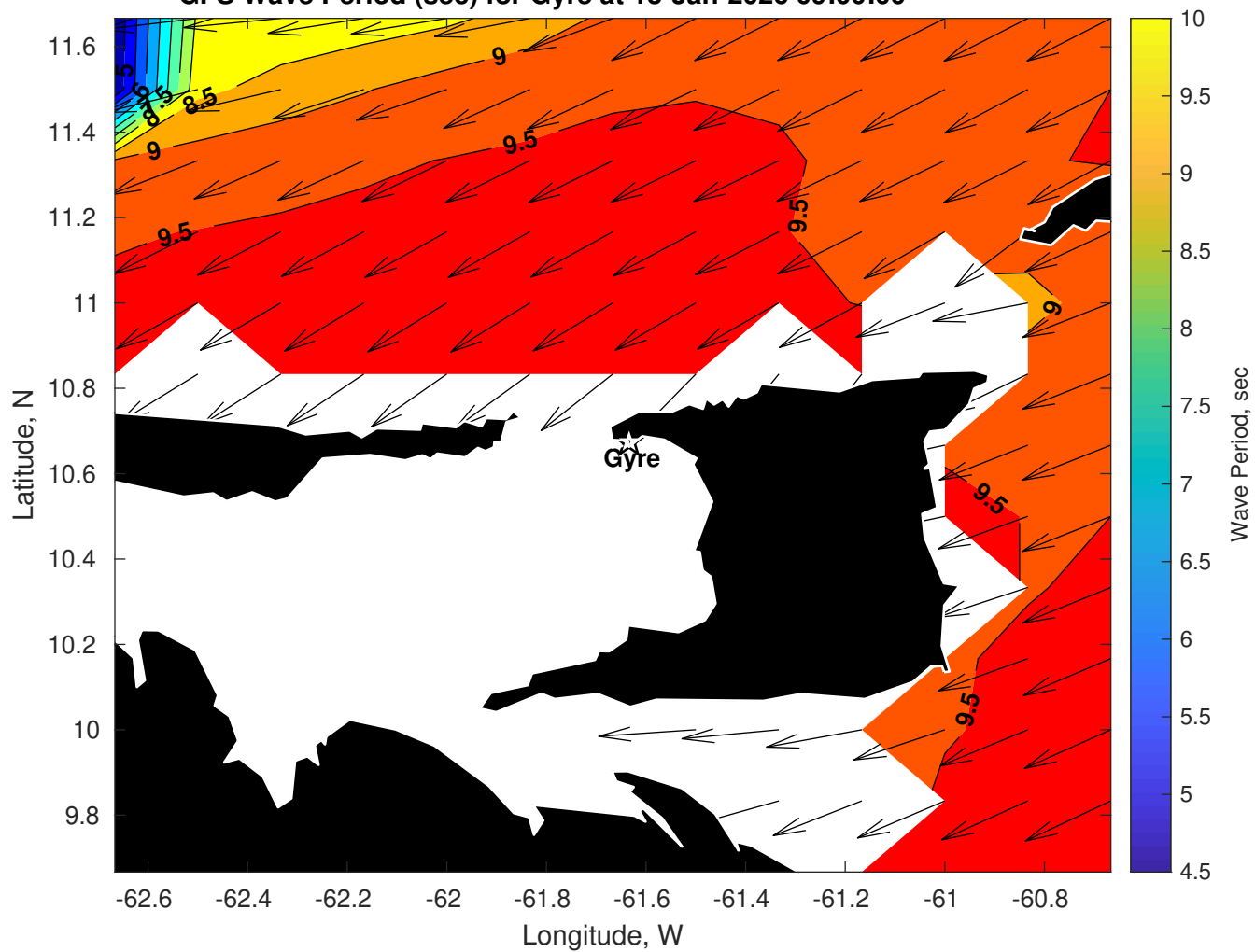
GFS Wave Period (sec) for Gyre at 13-Jan-2026 09:00:00
