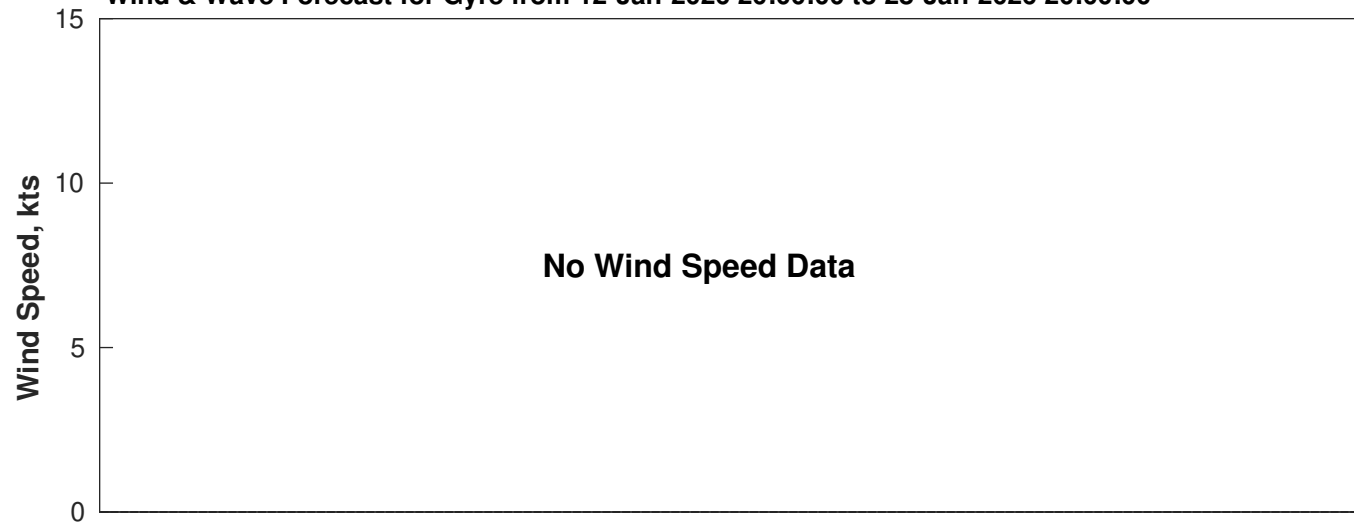
Wind & Wave Forecast for Gyre from 12-Jan-2026 20:00:00 to 28-Jan-2026 20:00:00
