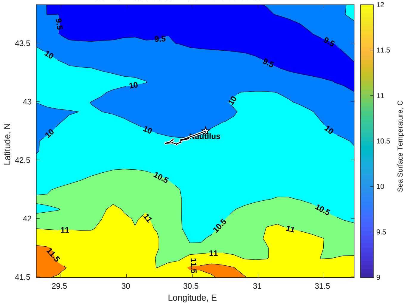
SST for Nautilus at 12-Jan-2026 00:00:00
