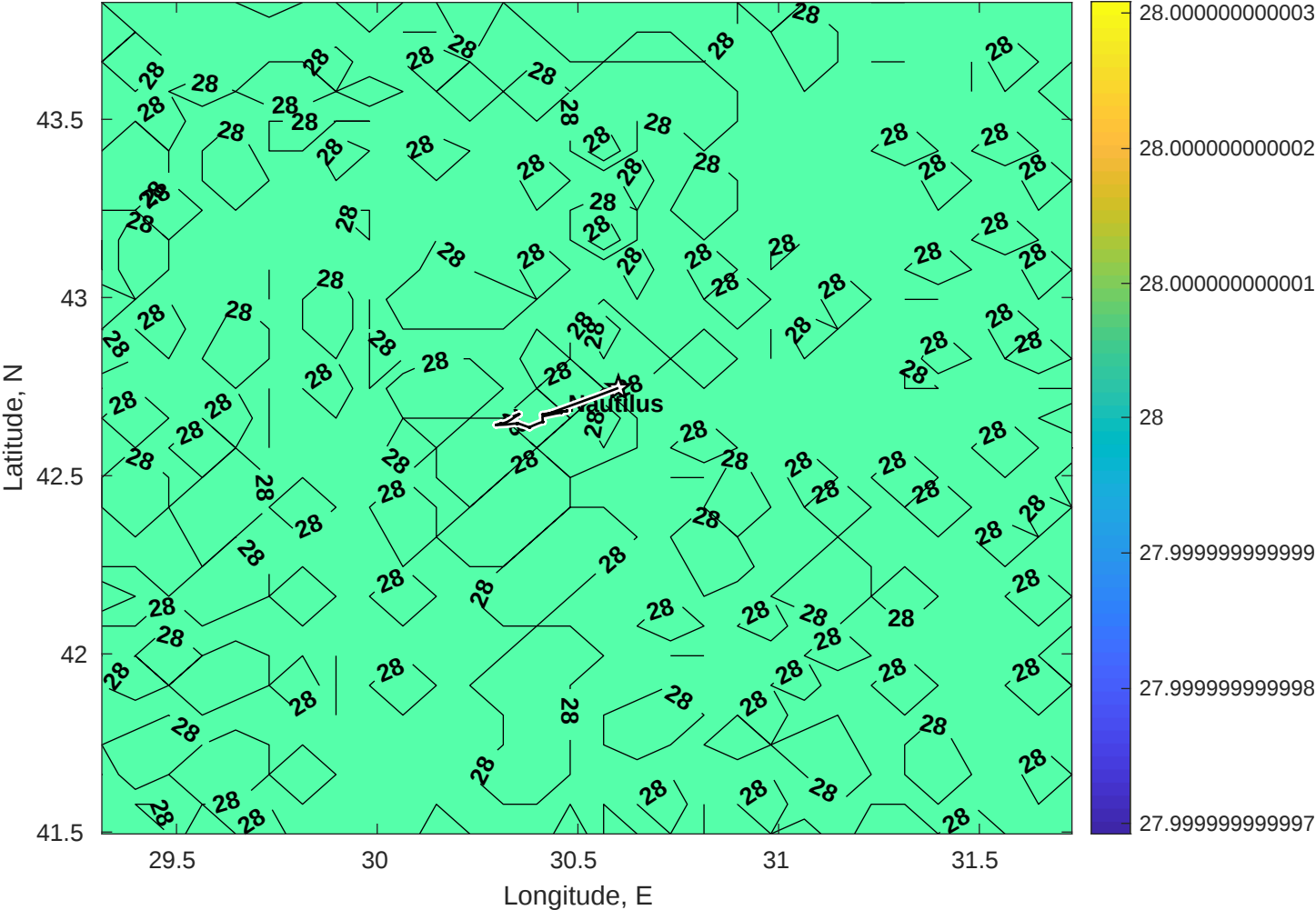
Surface Salinity for Nautilus at 12-Jan-2026 00:00:00
