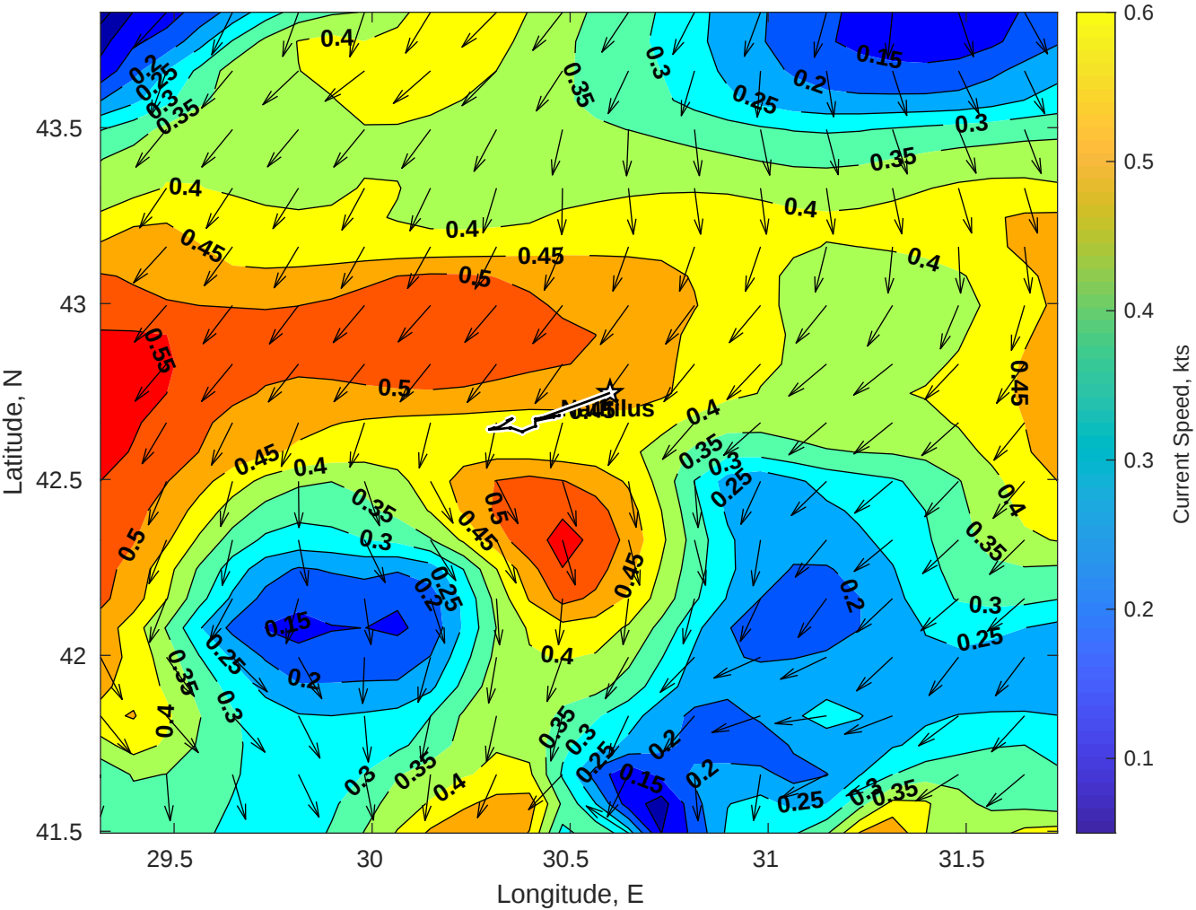
Surface Currents for Nautilus at 12-Jan-2026 00:00:00
