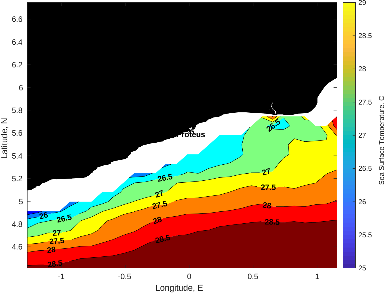
SST for Proteus at 12-Jan-2026 00:00:00
