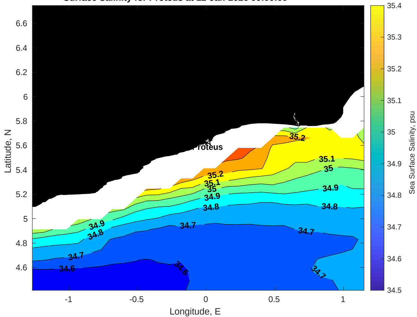
Surface Salinity for Proteus at 12-Jan-2026 00:00:00
