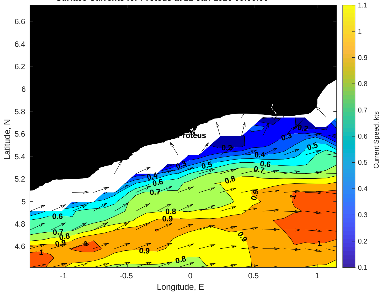
Surface Currents for Proteus at 12-Jan-2026 00:00:00
