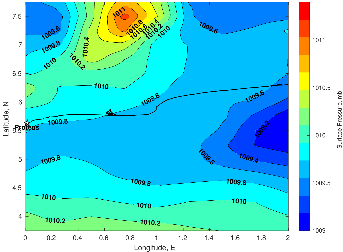
Surface Pressure (mb) for Proteus at 14-Jan-2026 00:00:00
