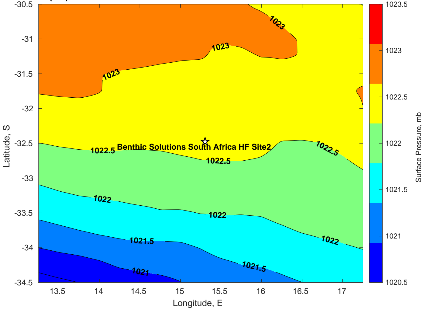
Surface Pressure (mb) for Benthic Solutions South Africa HF Site2 at 15-Jul-2025 12:00:00
