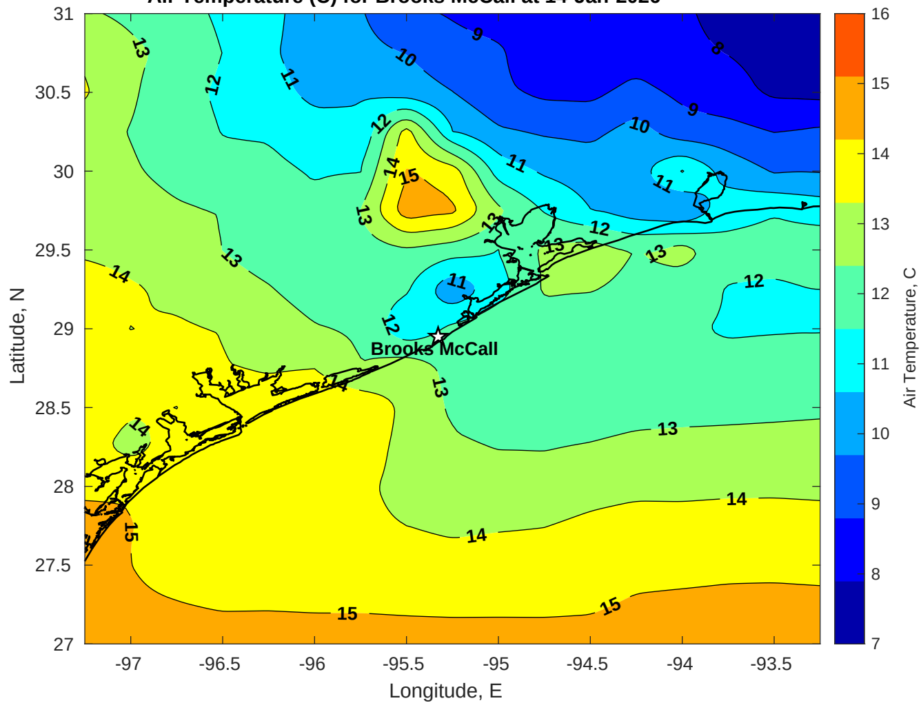
Air Temperature (C) for Brooks McCall at 14-Jan-2026
