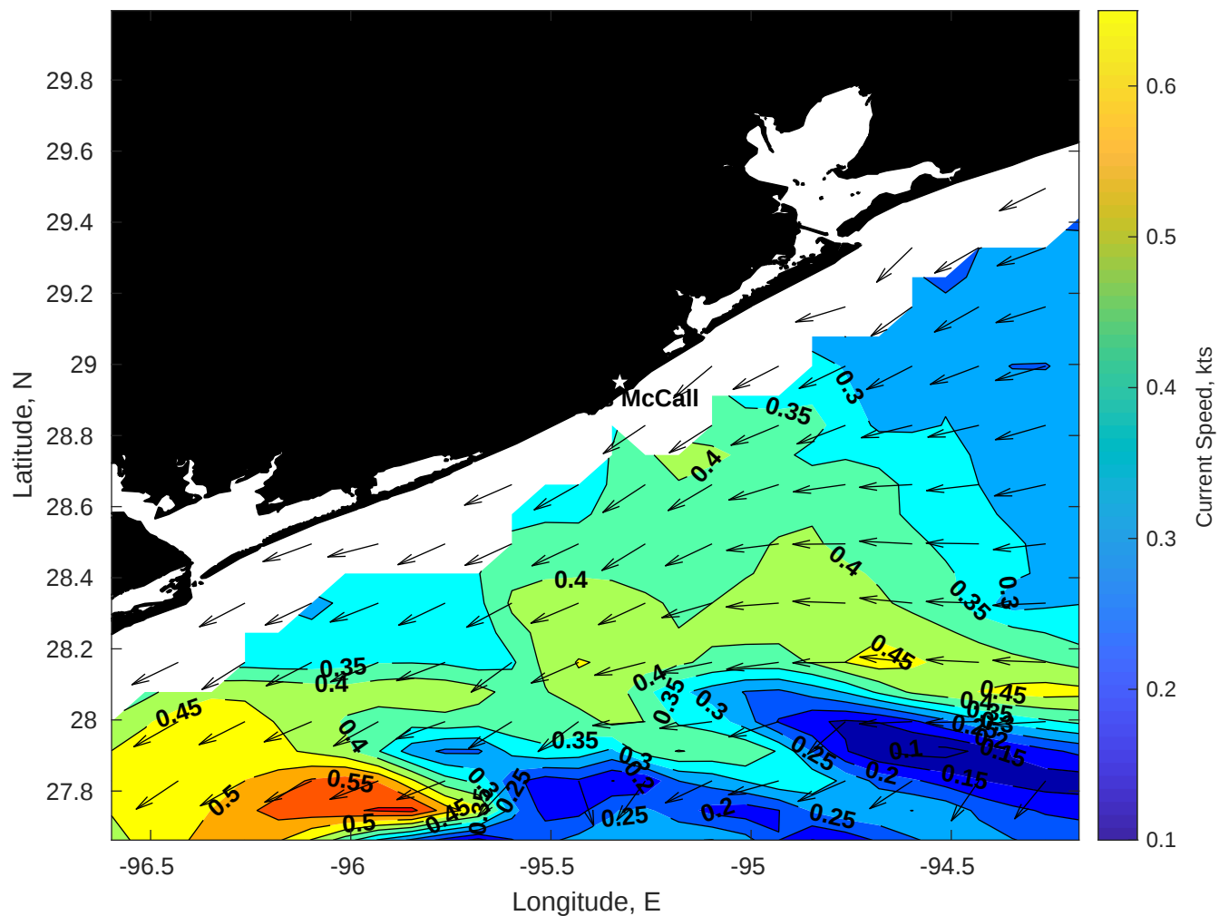
Surface Currents for Brooks McCall at 13-Jan-2026 00:00:00
