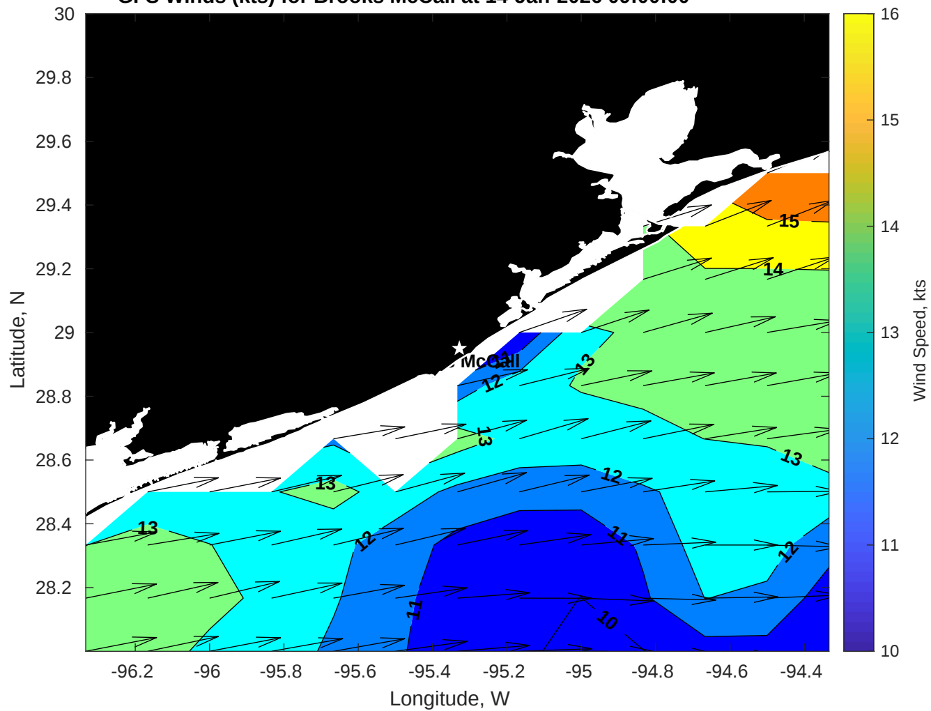
GFS Winds (kts) for Brooks McCall at 14-Jan-2026 09:00:00
