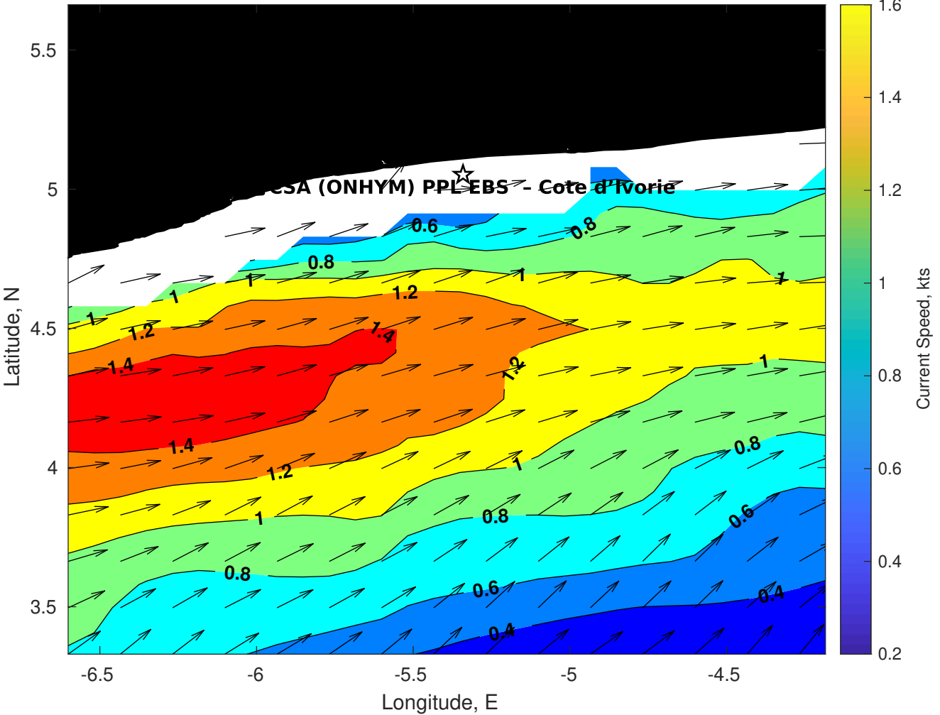
Surface Currents for CSA (ONHYM) PPL EBS - Cote d'Ivoire at 13-Jan-2026 00:00:00
