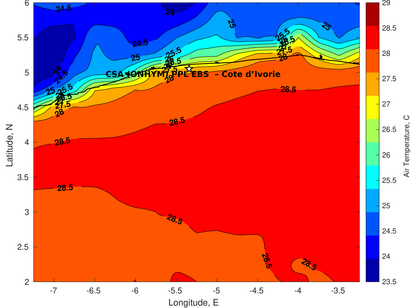
Air Temperature (C) for CSA (ONHYM) PPL EBS - Cote d'Ivoire at 14-Jan-2026
