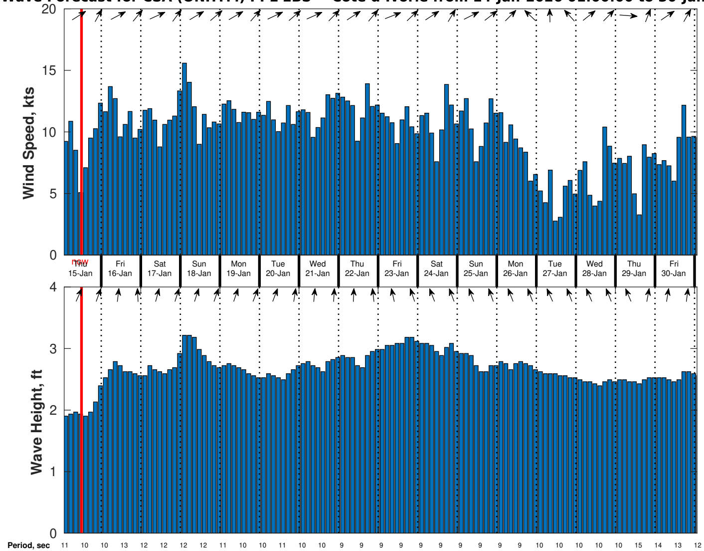
Wind & Wave Forecast for CSA (ONHYM) PPL EBS - Cote d'Ivoire from 14-Jan-2026 01:00:00 to 30-Jan-2026 01:00:00
