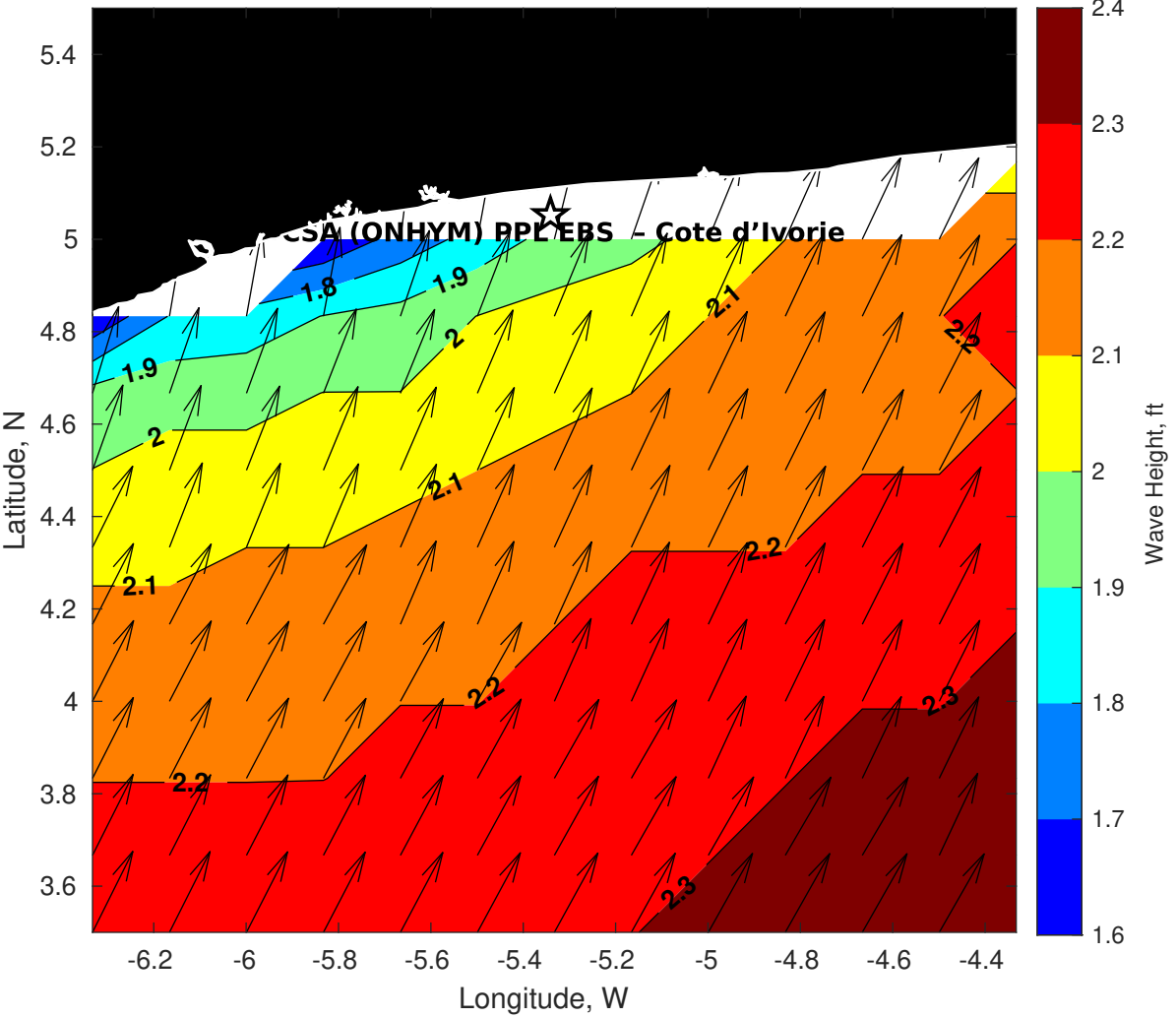
GFS Wave Height (ft) for CSA (ONHYM) PPL EBS - Cote d'Ivoire at 14-Jan-2026 09:00:00
