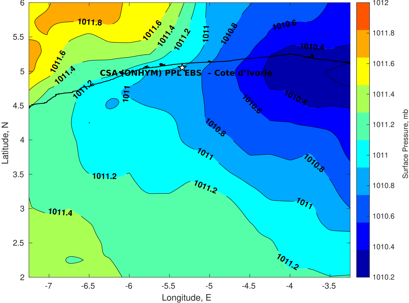
Surface Pressure (mb) for CSA (ONHYM) PPL EBS - Cote d'Ivoire at 14-Jan-2026 00:00:00
