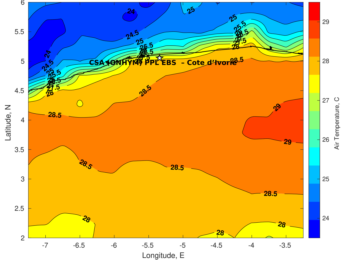
Air Temperature (C) for CSA (ONHYM) PPL EBS - Cote d'Ivoire at 14-Jan-2026
