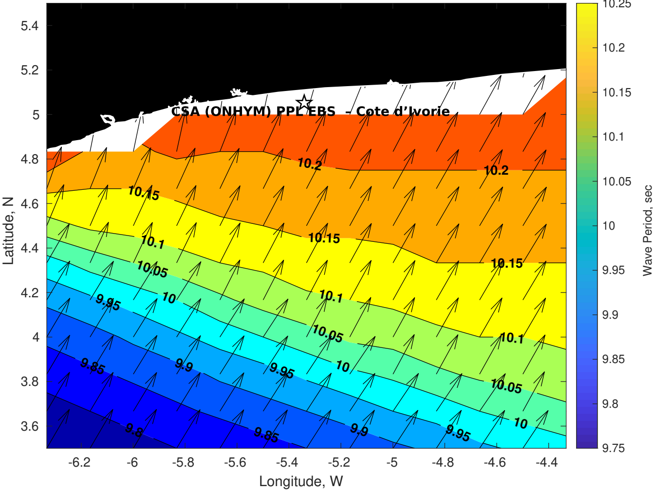
GFS Wave Period (sec) for CSA (ONHYM) PPL EBS - Cote d'Ivoire at 14-Jan-2026 09:00:00
