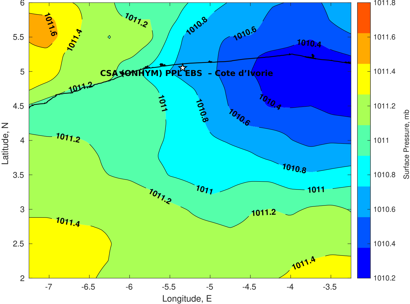
Surface Pressure (mb) for CSA (ONHYM) PPL EBS - Cote d'Ivoire at 16-Jan-2026 00:00:00
