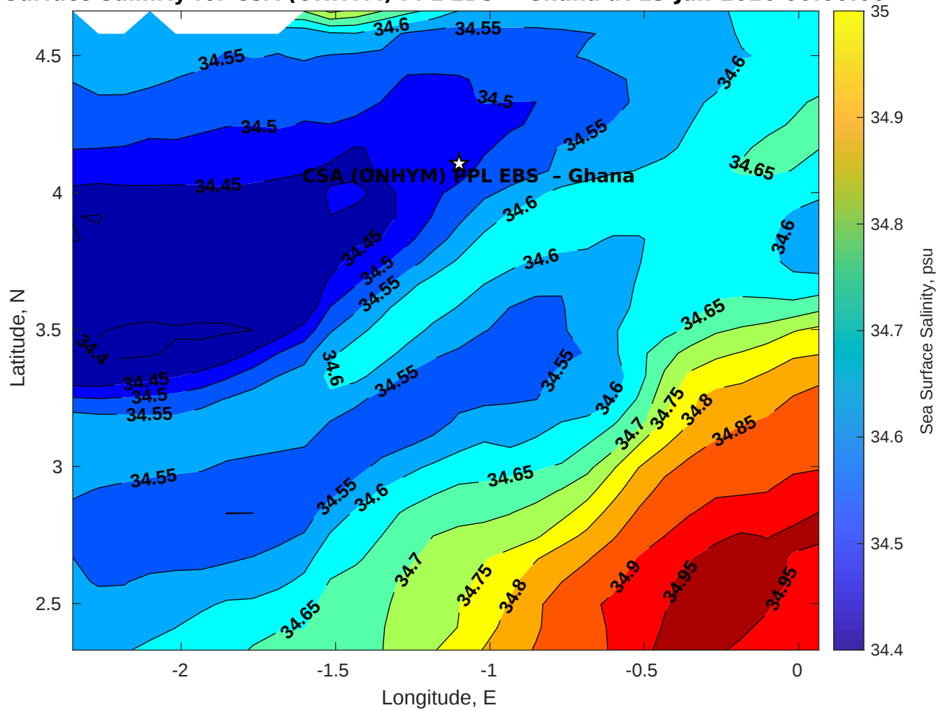
Surface Salinity for CSA (ONHYM) PPL EBS - Ghana at 13-Jan-2026 00:00:00
