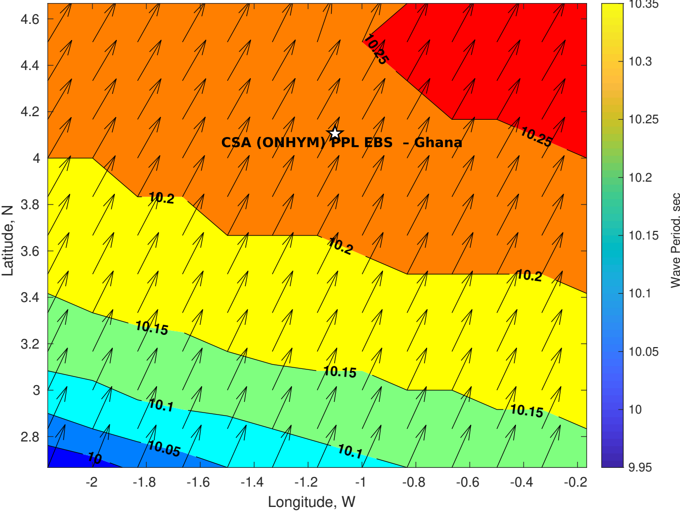
GFS Wave Period (sec) for CSA (ONHYM) PPL EBS - Ghana at 14-Jan-2026 09:00:00
