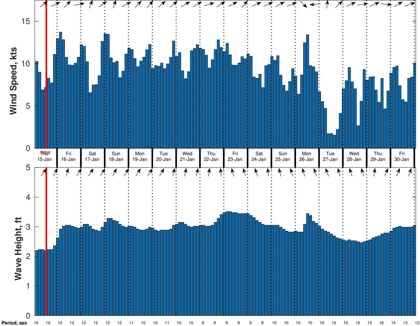
Wind & Wave Forecast for CSA (ONHYM) PPL EBS - Ghana from 14-Jan-2026 02:00:00 to 30-Jan-2026 02:00:00
