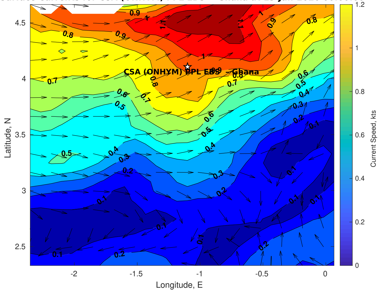
Surface Currents for CSA (ONHYM) PPL EBS - Ghana at 13-Jan-2026 00:00:00
