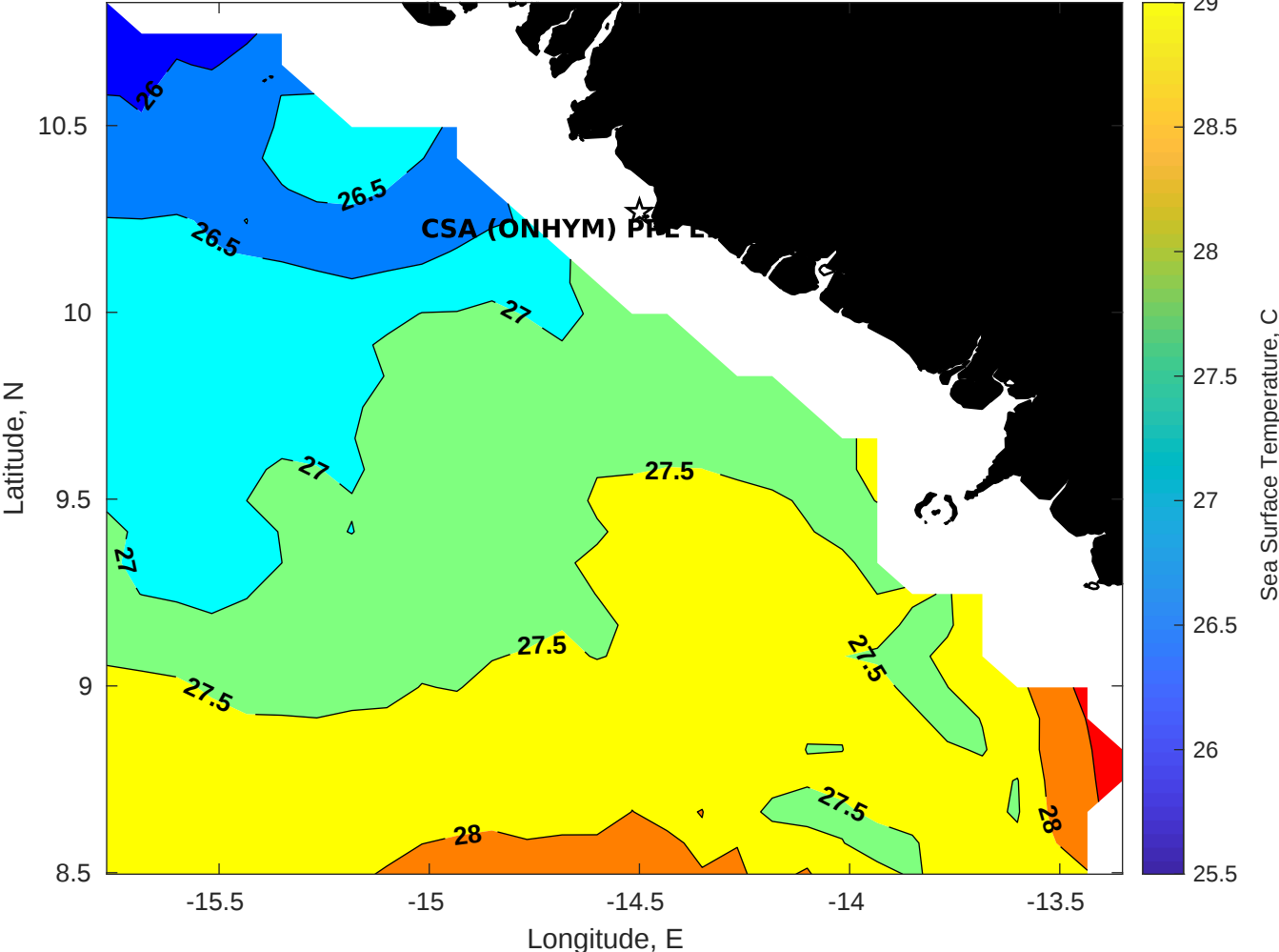
SST for CSA (ONHYM) PPL EBS - Guinea at 13-Jan-2026 00:00:00
