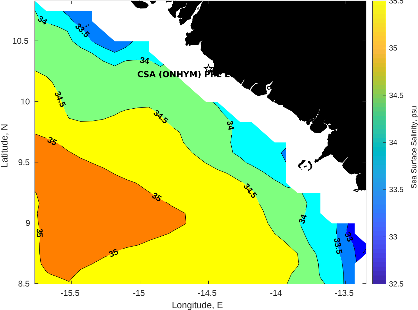
Surface Salinity for CSA (ONHYM) PPL EBS - Guinea at 13-Jan-2026 00:00:00
