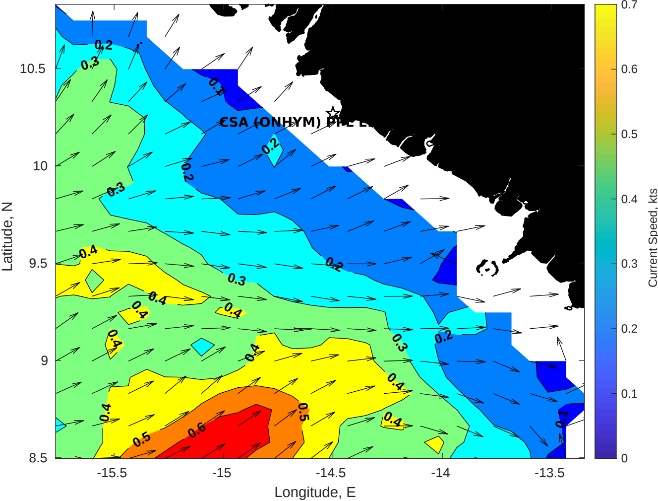
Surface Currents for CSA (ONHYM) PPL EBS - Guinea at 13-Jan-2026 00:00:00
