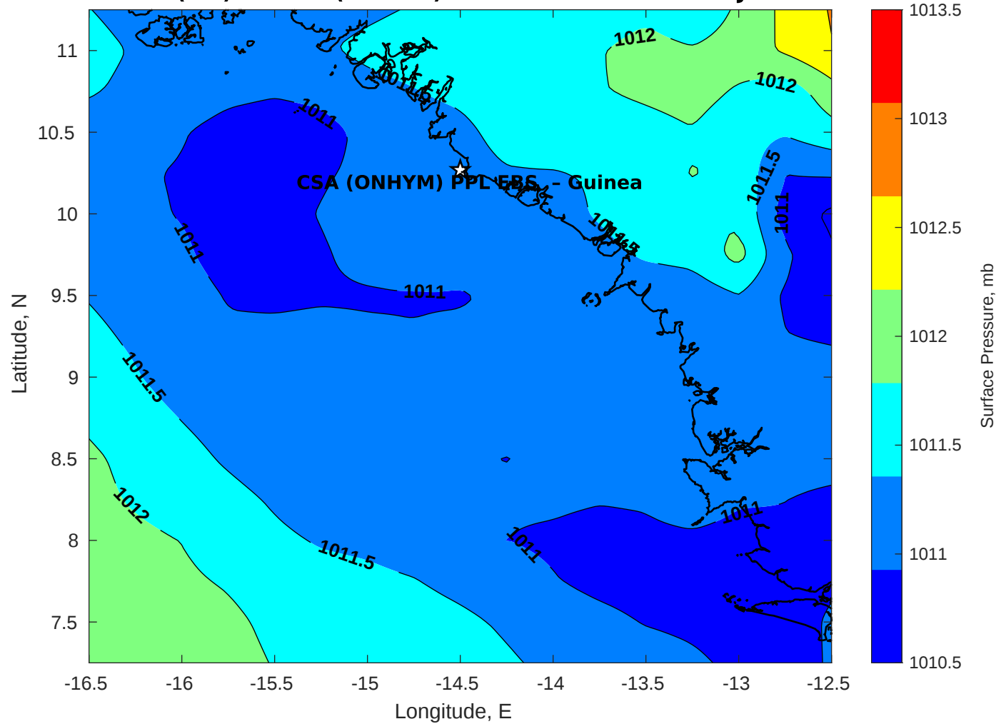
Surface Pressure (mb) for CSA (ONHYM) PPL EBS - Guinea at 15-Jan-2026 00:00:00
