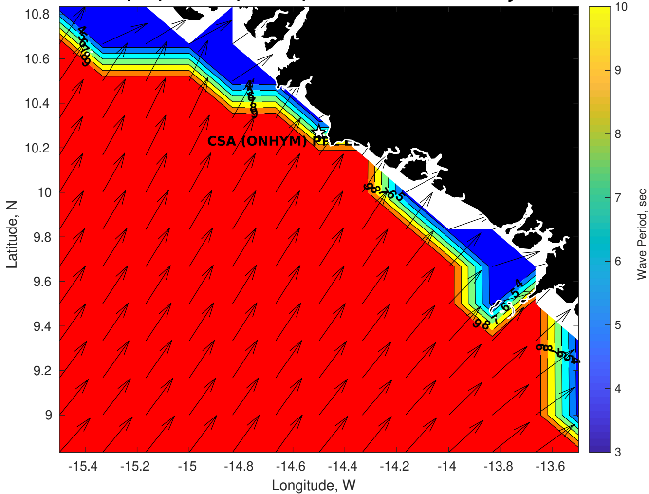
GFS Wave Period (sec) for CSA (ONHYM) PPL EBS - Guinea at 14-Jan-2026 09:00:00
