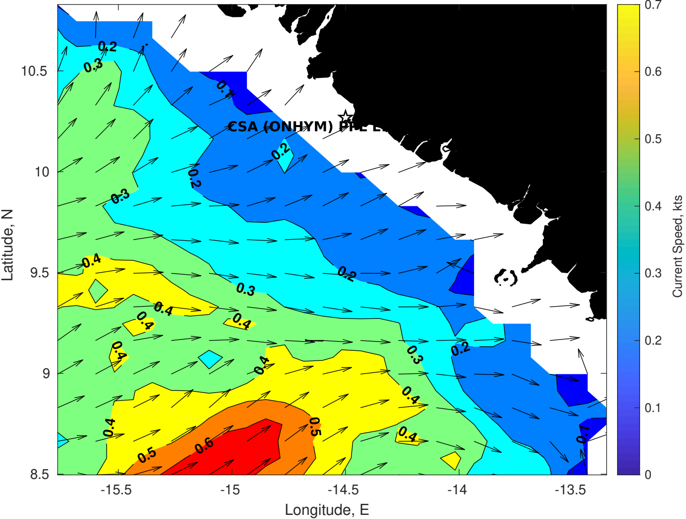
Surface Currents for CSA (ONHYM) PPL EBS - Guinea at 13-Jan-2026 00:00:00
