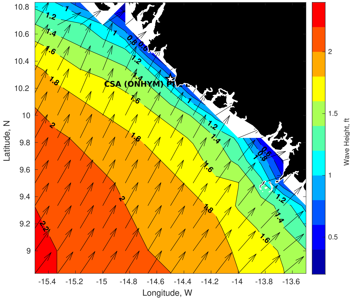
GFS Wave Height (ft) for CSA (ONHYM) PPL EBS - Guinea at 14-Jan-2026 09:00:00
