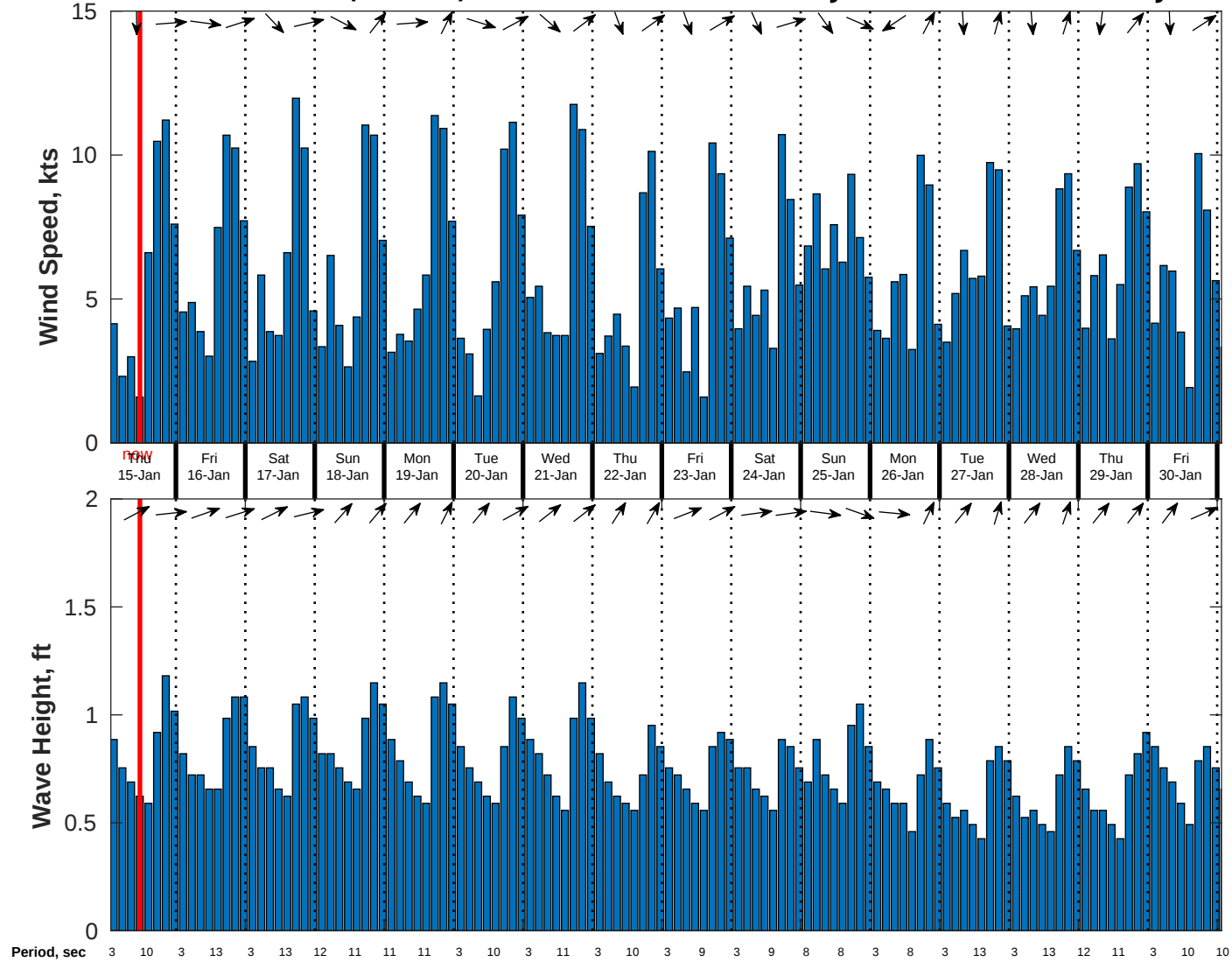
Wind & Wave Forecast for CSA (ONHYM) PPL EBS - Guinea from 14-Jan-2026 01:00:00 to 30-Jan-2026 01:00:00
